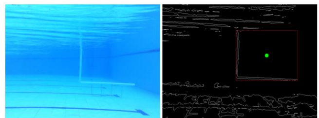
Figure 13: Localization of gate centre using contour validation
