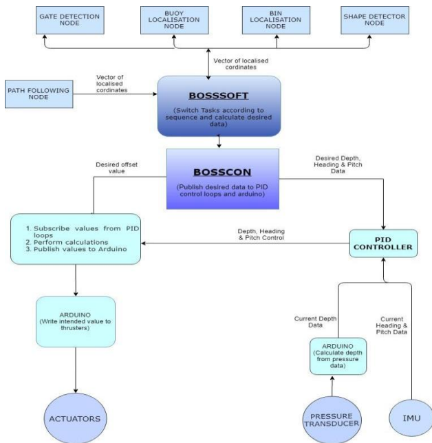
Figure 10: Software Framework of ARYA
