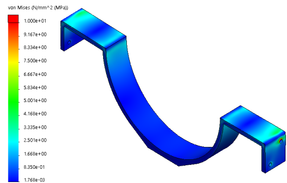
Figure 3: Stress Analysis of Frame
