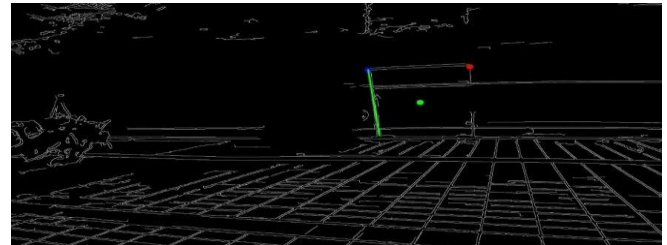
Figure 11: Gate Detection
