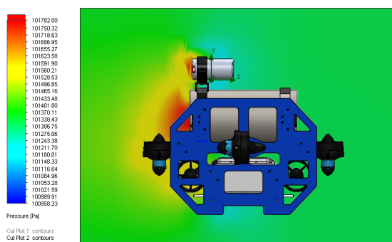
Figure 6: Pressure Contour for Surge Motion
