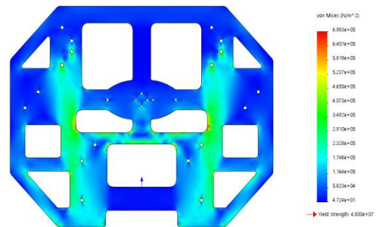
Figure 3: Stress Analysis of Frame
