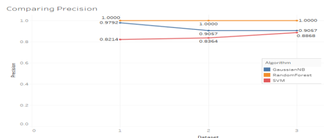
Fig4.Comparison of precision of algorithms across datasets
