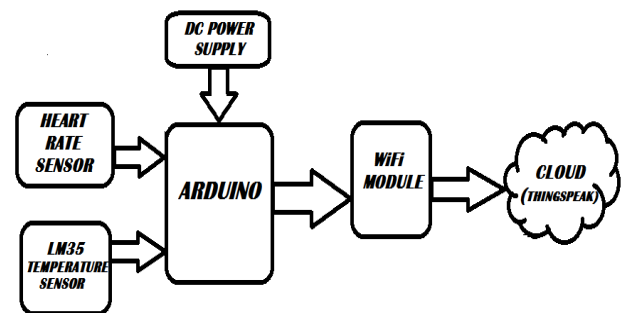
IOT BASED HEALTH MONITORING SYSTEM
