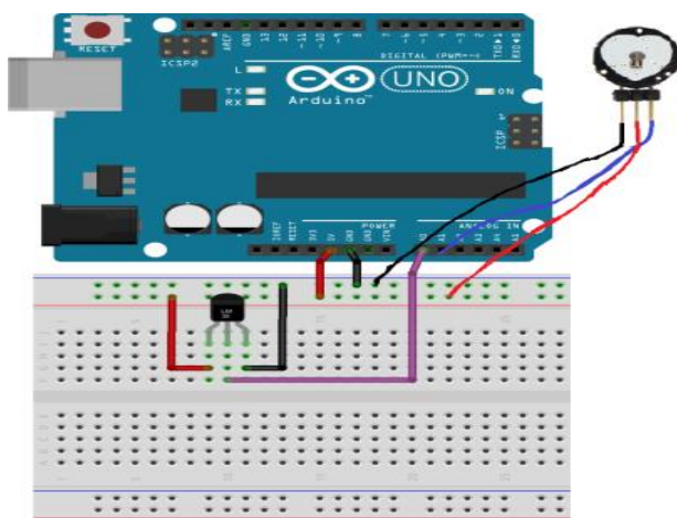
Fig 2. Diagram showing hardware interfacing between arduino and pulse sensor and temperature sensor
