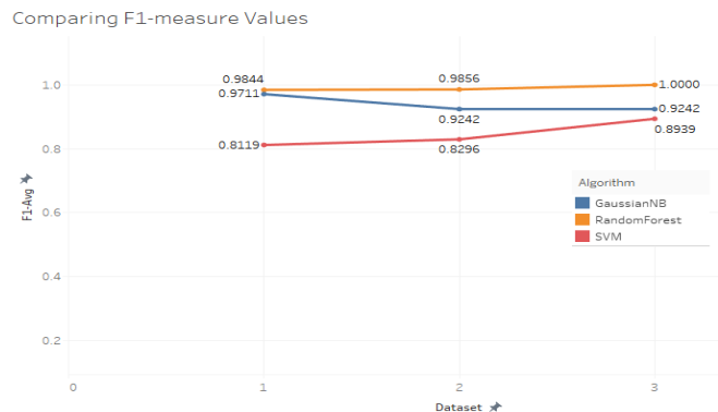
Fig 5. Comparison of F1-measures of different algorithms across datasets
