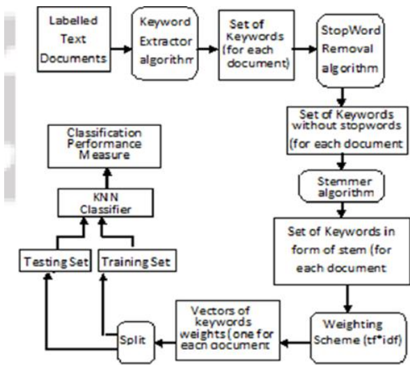
Figure 1: Flow of text classification
