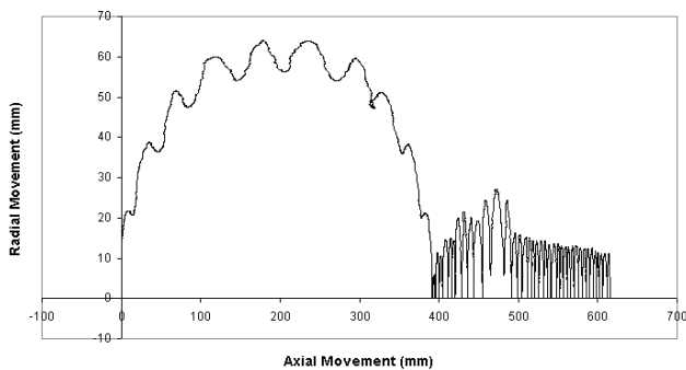
Fig. 4 particle Movement in 3-phase GIB (400KV/Al / 0.1mm / 10mm / 1° Monte-Carlo technique)
