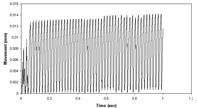
Fig. 7 : particle Movement in 3-phase GIB on coated electrodes (400KV/Cu / 0.1mm / 10mm / 50 micro meter)
